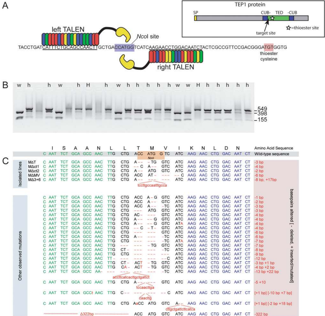
Figure 1. TALEN mutagenesis of the TEP1 gene. A: Fragment from the TEP1 gene showing the target site of the TALEN pair. Nucleotides bound by each TALEN are underlined, TALEN repeats are color-coded to show repeat/nucleotide specificity. The NcoI restriction site centrally located at the TALEN cleavage site is highlighted. Inset: scheme of the entire TEP1 protein showing the location of TALEN-induced mutations (SP: signal peptide; CUB: CUB domain interrupted by the TED: thioester domain; the star indicates the position of the thioester site). B: PCR assay to identify TEP1 mutant mosquitoes. A PCR product spanning the TALEN target site is generated from individual mosquitoes (small larva or a leg from a living adult) and incubated with NcoI. Full cleavage of the PCR product (w) denotes a wild-type individual. Partial cleavage (h) denotes a heterozygous TEP1 mutant. Absence of cleavage (H) corresponds to a homozygous TEP1 mutant. C: TALEN-induced mutations in the TEP1 gene. Left and right TALEN target nucleotide sequences are shown in green and blue respectively, with the 15bp spacer sequence between the TALENs in black. The NcoI restriction site is highlighted in orange. Deletions are designated by a red dash or by Δ+number of missing bases. Insertions are shown in lowercase red letters. Uppercase red letters correspond to natural polymorphisms between multiple TEP1 alleles.
