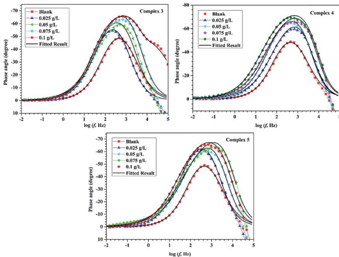
Fig. 8 Phase angle plots of mild steel in 15% M HCl solutions without and with various concentrations of inhibitor.
