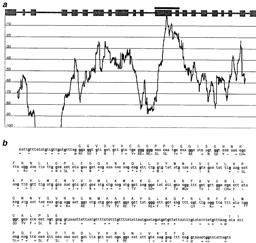
Figure 2. Optimal amplicon selection for deleterious mutation discovery. a, Graphical representation of the relative susceptibility of each 500-bp amplicon to C/G to T/A transitions causing a deleterious mutation in the Arabidopsis CMT3 gene. Exons are indicated as shaded boxes above the plot. Each point on the plot is the sum of scores calculated for a 500-bp amplicon window centered at that residue. A residue susceptible to a nonsense change scored +6, to a missense change scored 0, to a silent change scored -1, and to a splice junction mutation scored +4. The scoring system is based on the potential overall frequency of these changes in genes of Arabidopsis. Bar delimits region analyzed in b. b, Sites that are susceptible to the C/G to T/A transition mutations are indicated under the DNA sequence for the amplicon. Each amino acid of the coding sequence is indicated above its codon. The consequence for each mutation is indicated below. Letters indicate a missense change, = indicates a silent change, * indicates a nonsense change, and phi indicates a splice site mutation.
