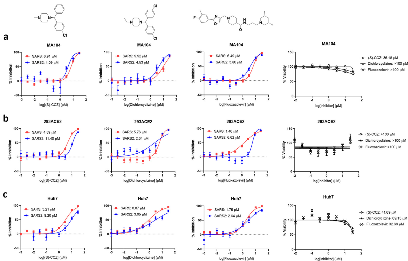
FIG 1 (S)-CCZ, dichlorcyclizine, and fluoxazolevir inhibit human CoV S-mediated infection. The chemical structures of (S)-CCZ, dichlorcyclizine, and fluoxazolevir are shown on the top. SARS-CoV and SARS-CoV-2 pseudotyped virus infection and cytotoxicity (right) assays were performed in MA104 (a), 293ACE2 (b), and Huh7 (c) cells with (S)-CCZ, dichlorcyclizine, and fluoxazolevir, with dimethyl sulfoxide (DMSO) as a control (see Materials and Methods). Luminescent signals were measured using a POLARstar Omega plate reader. EC_{50} and CC_{50} values were calculated using Prism 7 software. Each data point is presented as mean values \pm standard errors of the means ( n = 6 to 8 biological independent replicates). All results are representative of three independent experiments.
