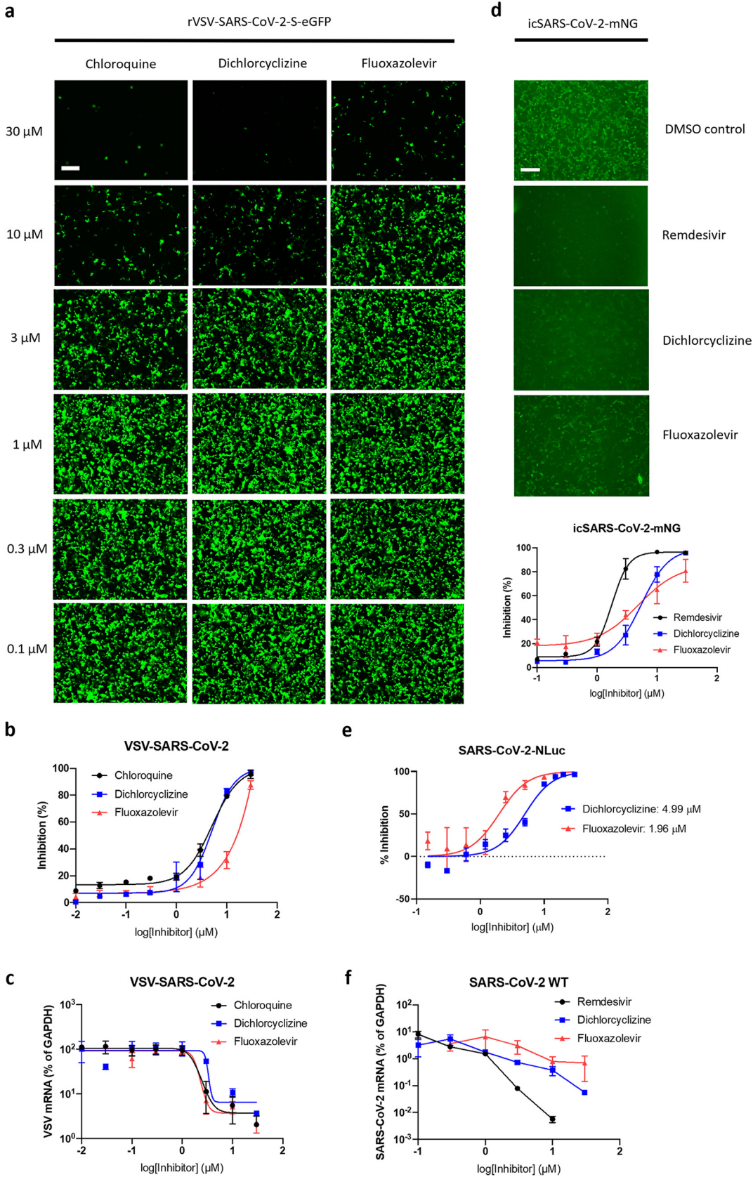
FIG 2 Dichlorcyclizine and fluoxazolevir suppress wild-type SARS-CoV-2 infection. (a to c) MA104 cells were treated with chloroquine, dichlorcyclizine, and fluoxazolevir at the indicated concentrations for 1 h and infected with rVSV-SARS-CoV-2-S-eGFP (Continued on next page)
