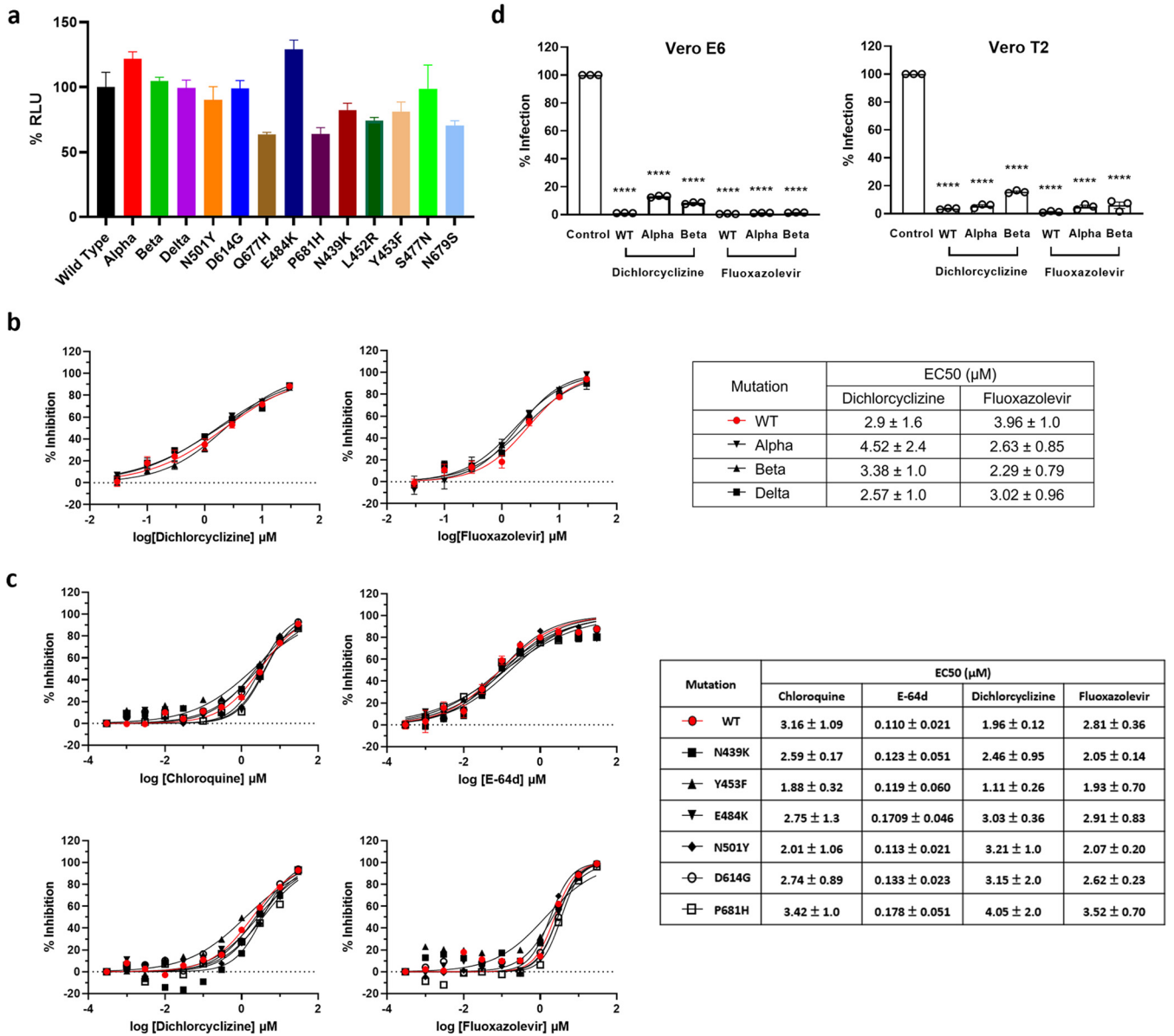
FIG 3 Efficacy of dichlorcyclizine and fluoxazolevir against SARS-CoV-2 variants. (a) VSV-SARS-CoV-2-S pseudotyped virus containing N439K, L452R, Y453F, S477N, E484K, N501Y, D614G, Q677H, N679S, or P681H mutation was generated. VSV L mRNA levels were measured to calculate genome copy numbers per volume of pseudotyped VSV stock. The cells were then infected with the same multiplicity of infection, and luminescent signals were measured using a POLARstar Omega plate reader. Each data point is presented as mean values \pm SEM ( n = 6 to 8 biological independent replicates). (b) VSV-SARS-CoV-2-S pseudotyped viruses containing mutations appearing in alpha, beta, and delta variants were generated and tested against dichlorcyclizine and fluoxazolevir in Huh7 cells. Luminescent signals were measured using a POLARstar Omega plate reader 24 h after infection. EC 50 values are calculated using Prism 7 software and shown in the table on the right. Each data point is presented as mean values \pm SEM ( n = 6 to 8 biological independent replicates). (c) VSV-SARS-CoV-2-S pseudotyped viruses containing N439K, Y453F, E484K, N501Y, D614G, or P681H mutations were tested against (S)-CCZ, dichlorcyclizine, and fluoxazolevir in Huh7 cells. Luminescent signals were measured using a POLARstar Omega plate reader. EC 50 values are calculated using Prism 7 software and shown in the table on the right. Each data point is presented as mean values \pm SEM ( n = 6 to 8 biological independent replicates). (d) Vero E6 and Vero T2 cells were infected with wild-type, alpha, and beta variants at a multiplicity of infection of 0.1 with or without 10 \mu M the compounds. At 16 h postinfection, SARS-CoV-2 RNA was measured using primers targeting N. Relative levels of the viral genome were calculated using the GAPDH gene as a normalization control. The data are presented as means \pm SD (three independent replicates). All results are representative of three independent experiments.
