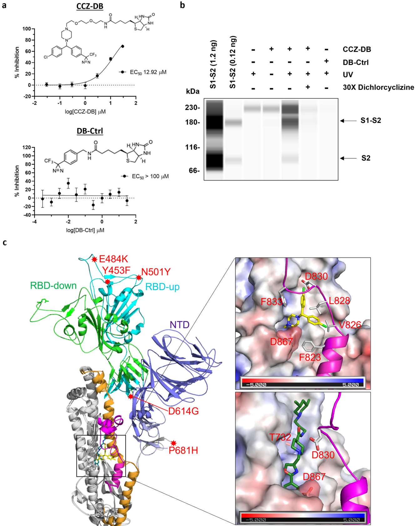
FIG 5 Antiviral mechanism of dichlorocyclizine and fluoxazolevir against SARS-CoV-2. (a) Structures and dose-response curves of CCZ-DB and DB-Ctrl. CCZ-DB was active in inhibiting pseudotyped VSVs harboring SARS-CoV-2 S, with an EC_{50} of 12.92 \mu M . The DB-Ctrl has the diazirine-biotin moieties but was not (Continued on next page)
