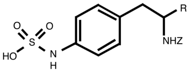
Figure 2. The core structure of AKB-9778 (p-substituted phenylsulfamic acid).
