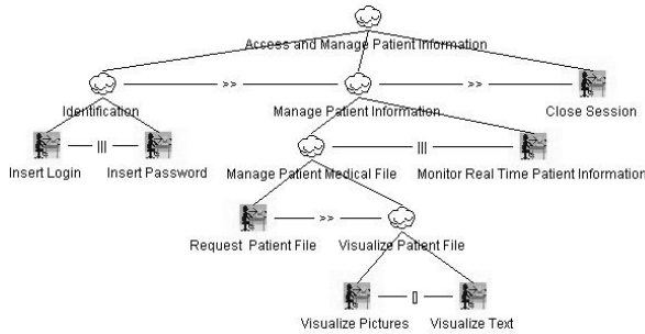
Fig. 6. The CTM for the nurse using a handheld PC.
