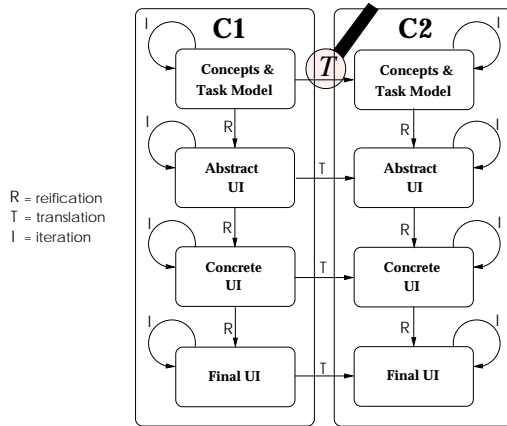
Fig. 1. The reference development process for supporting context-sensitive UIs ([1]).
