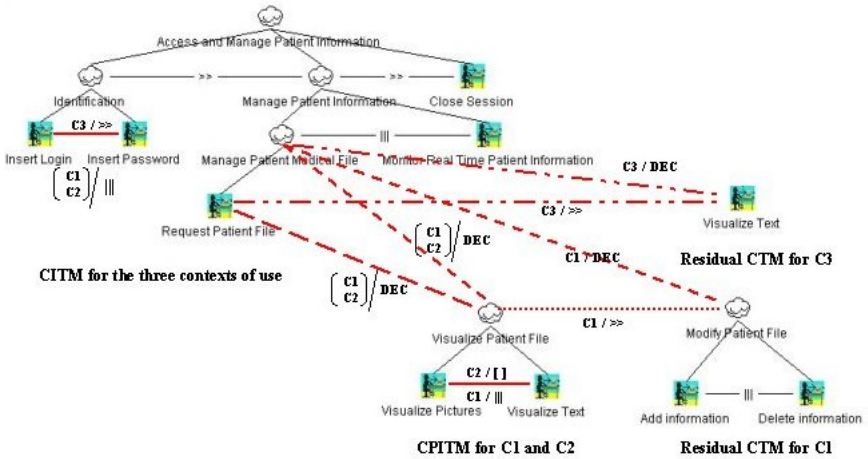
Fig. 10. Multi-Context Task Model for the Case Study.
