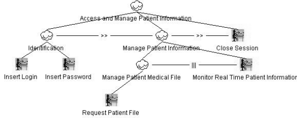
Fig. 8. The CITM for the three different contexts of use.
