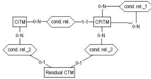
Fig. 3. Multi-Context Task Model concepts.
