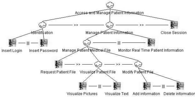
Fig. 5. The CTM for the doctor using a desktop PC.
