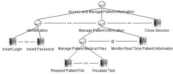
Fig. 7. The CTM for the doctor using a Cellular Phone.
