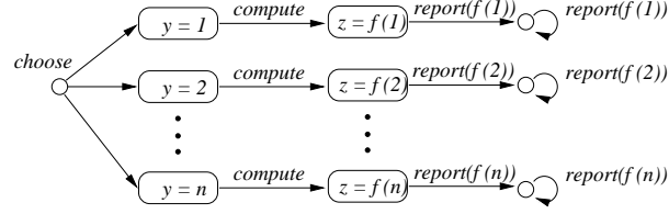
Figure 8: Task-PIOA Trapdoor
