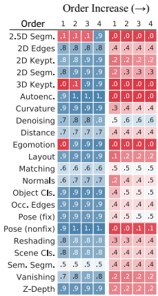
Figure 10: Generalization to Novel Tasks. Each row shows a novel test task. Left: Gain and Quality values using the devised “all-for-one” transfer policies for novel tasks for orders 1-4. Right: Win rates (%) of the transfer policy over various self-supervised methods, ImageNet features, and scratch are shown in the colored rows. Note the large margin of win by taxonomy. The uncolored rows show corresponding loss values.
