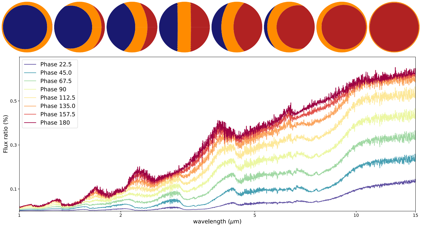
Figure 4. Top: geometry of the phase model at different phases. From left to right: 22.5, 45, 67.5, 90, 112.5, 135, 157.5, and 180. Blue: night-side contribution; orange: terminator contribution; red: day-side contribution. Bottom: corresponding phase-curve emission from our model.
