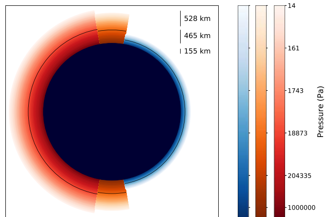
Figure 6. Geometry of our phase-curve model showing the three different altitude–pressure profiles. Red: day side; orange: terminator region; blue: night side. The strength of the color represents the pressure. For indication, we also show with the black solid line the altitude at 5H , where H is the averaged scale height. The corresponding altitude values in kilometers are indicated in the top-right corner.
