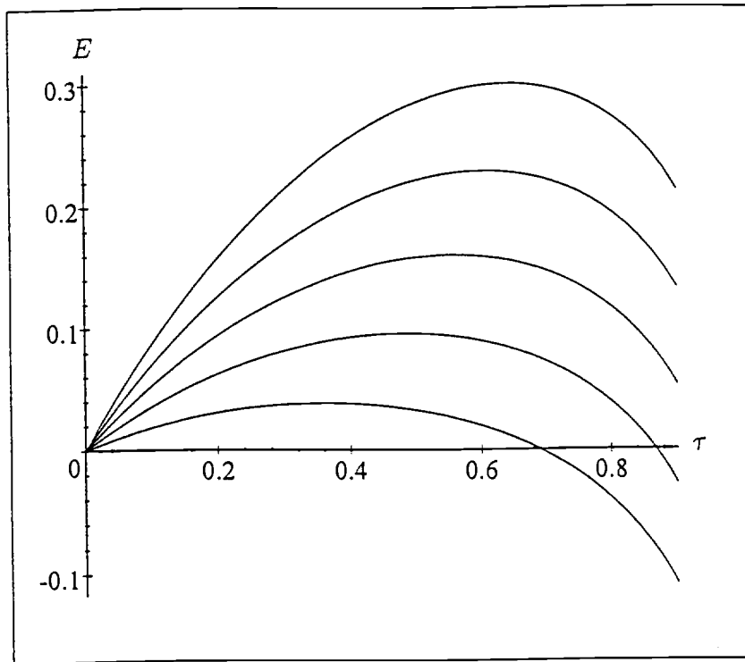
Figure 6. Efficiency, for 1 - r = 0, 1, 2, 3, 4 (bottom to top)
