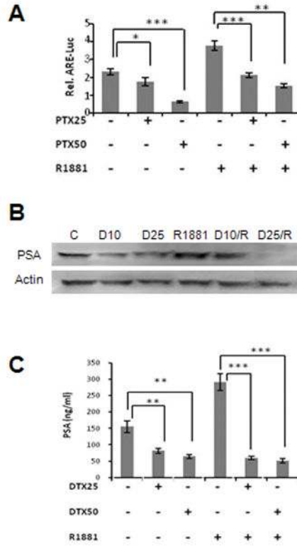
Figure 2. AR transcriptional activity is inhibited by taxane treatment
