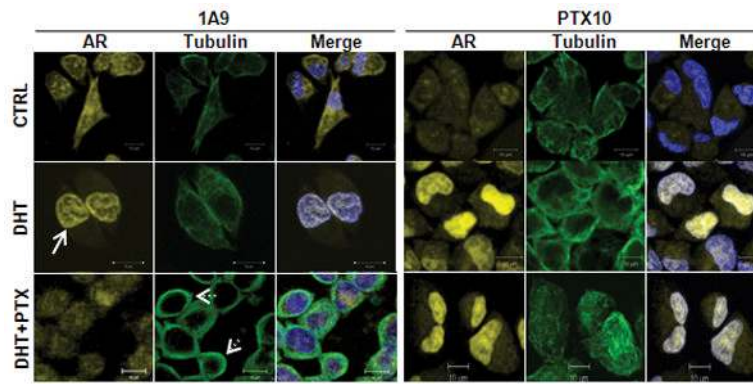
Figure 3. Taxane-induced AR cytoplasmic sequestration requires microtubule stabilization Paclitaxel treatment has no effect on AR subcellular localization in \beta -tubulin mutant paclitaxel-resistant cells. Parental, 1A9, and paclitaxel-resistant 1A9/PTX10 ovarian cancer cells were stably transfected with GFP-AR, treated for 2hr with either DMSO or 100nM PTX followed by the addition of 100nM DHT for another 2hr. Cells were then fixed, stained for AR, tubulin and DAPI and imaged by point scanning confocal microscopy. Solid arrows: nuclear AR; dashed arrow: microtubule bundles
