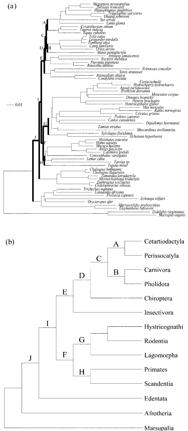
FIGURE 2. Model tree for the simulations based on the Eutherian mammal tree from Murphy et al. (2001) and Eizirik et al. (2001). (a) Full 66-taxon tree; interordinal relationships are represented by thick branches designated with letters. (b) Phylogenetic relationships of the mammalian orders present in the model tree.
