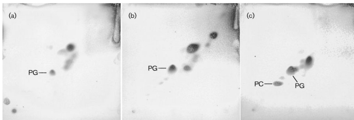
Fig. 2. Two-dimensional thin-layer chromatograms of the polar lipids of B. marina (a), Pirellula staleyi (b) and R. baltica (c). All polar lipids were stained with 5% (v/v) ethanolic molybdophosphoric acid. Solvents: chloroform/methanol/water (65:25:4, by vol.), first dimension; chloroform/methanol/acetic acid/water (80:12:15:4, by vol.), second dimension. Unlabelled lipids could not be fully characterized or assigned to known structures. PG, Phosphatidylglycerol; PC, phosphatidylcholine.
