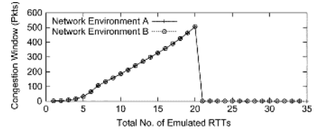
Fig. 14. Valid trace with “Remaining at 1 Packet.” That is, the window size remains at 1 packet after the timeout.
