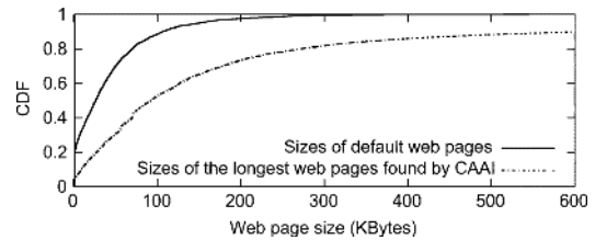
Fig. 7. CDF of the sizes of the default Web page and the longest Web pages found by CAAI.
