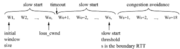
Fig. 8. Valid trace of window sizes.
