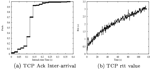
Figure 3: 3G Link Delay Variability
