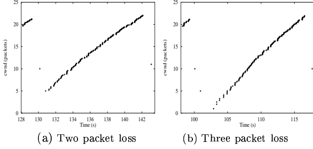
Figure 5: Congestion Window with multiple losses
