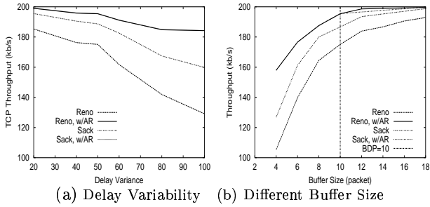
Figure 11: Throughput with Variable Delay e(x)+400 \cdot x
