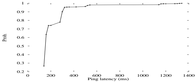
Figure 2: CDF of Ping Latencies
