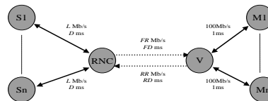
Figure 10: Simulation Topology
