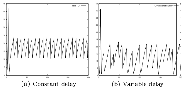
Figure 4: TCP Congestion Window Evolution over time
