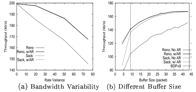
Figure 12: Throughput with Variable Bandwidth u(200, x)
