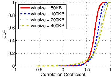
Figure 4: Distribution of correlation coefficients of RTGs
