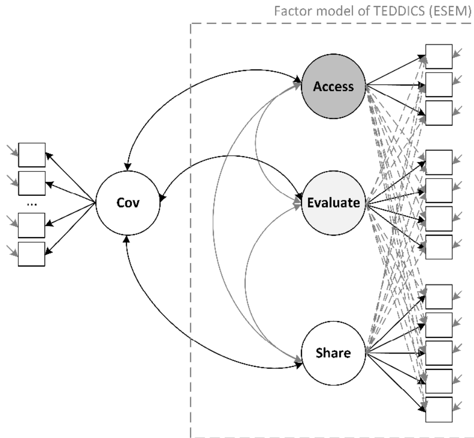
Figure 2. Exploratory structural equation model describing the relations between TEDDICS and another construct (Covariate, Cov ). Access = Accessing digital information, Evaluate = Evaluating digital information, Share = Sharing and communicating digital information.
