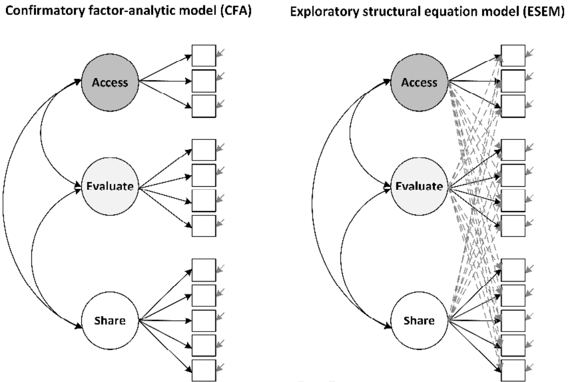
Figure 1. Factor-analytic models describing the structure of TEDDICS. Access = Accessing digital information, Evaluate = Evaluating digital information, Share = Sharing and communicating digital information.
