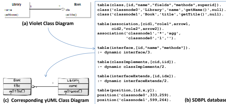
Fig. 13. A Violet Diagram mapped to an SDBPL database mapped to a yUML Diagram.
