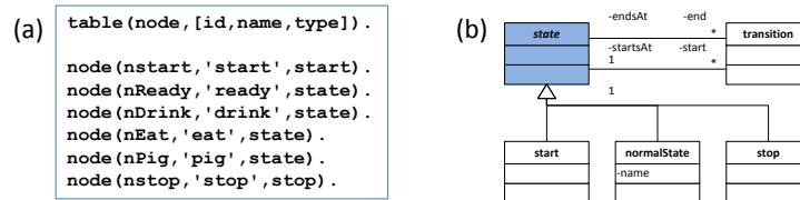
Fig. 5. A Prolog Table and Target MetaModel.
