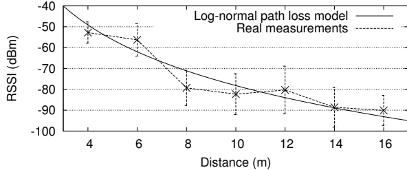
Figure 7. In the archaeological site, the CC2420 RSSI tends to follow the log-normal path loss model when drones are in flight.
