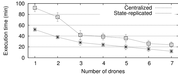
Figure 8. Using multiple drones provides significant improvements in execution time.
