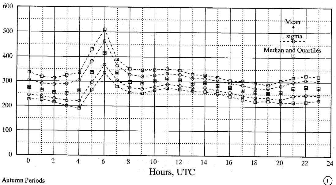
Fig. 1e,f. Seasonal median and mean of the evaluated slab thickness (km) derived from TEC and f_0F_2 measurements (see eq. (2.2)). Mean, mean minus standard deviation \sigma , mean plus \sigma are marked by circles. Median, and quartiles are marked by squares. The figures refer respectively to: e) data of May, June, July; f) data of August, September, October.
