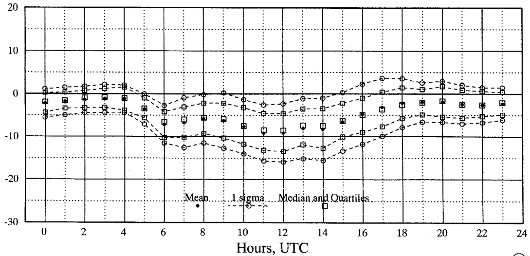
Fig. 2e,f. Seasonal median and mean of the differences between TEC modelled by eq. (4.1) and TEC derived from Faraday measurements. The legenda «fixed slope» means that eq. (4.1) has been used with constant \tau = 230 km for all the periods (see text). Mean, mean minus standard deviation \sigma , mean plus \sigma are marked by circles. Median, and quartiles are marked by squares. The figures refer respectively to: e) data of May, June, July; f) data of August, September, October.
