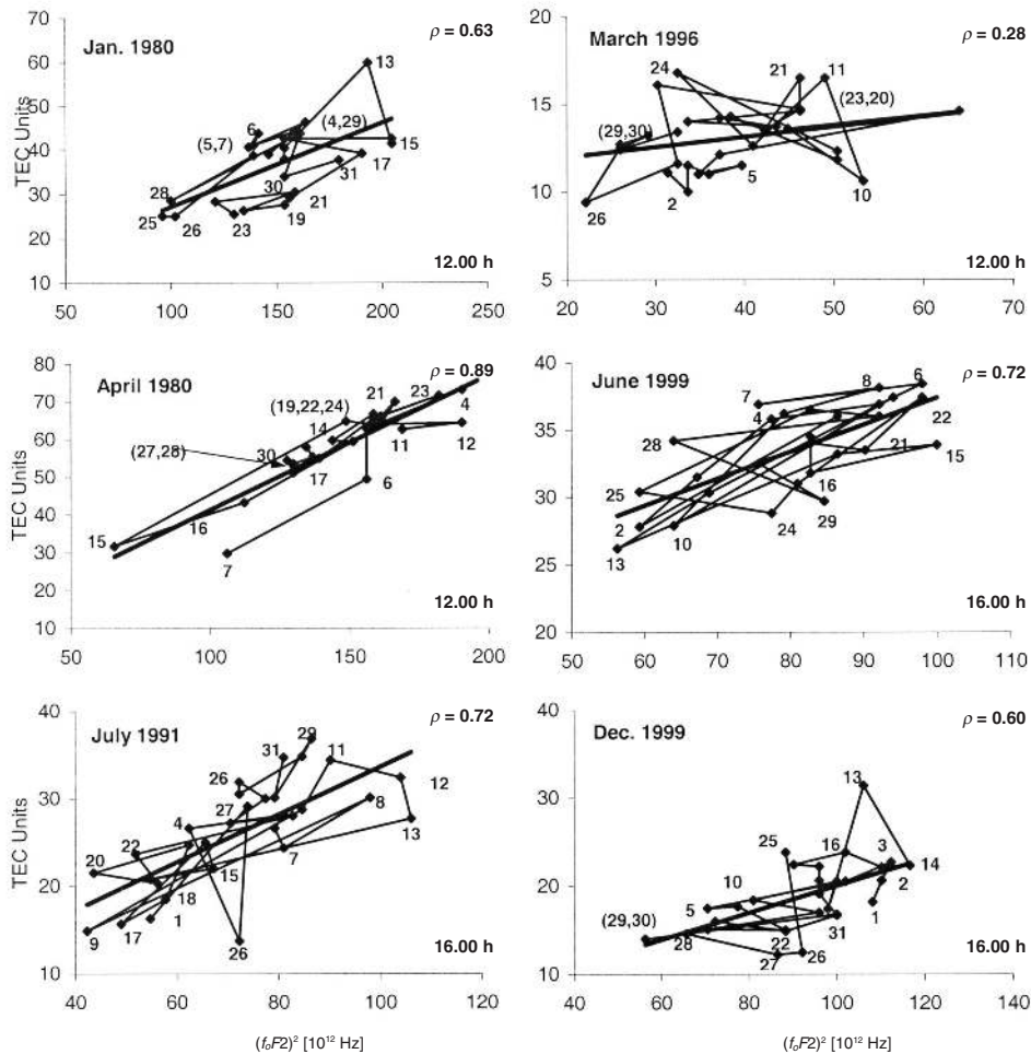
Fig. 3. Linear correlation between TEC Faraday rotation ( left ), GPS ( right ) and (f_oF2)^2 hourly daily values at some selected months/years, at given hours (12.00 or 16.00 h).
