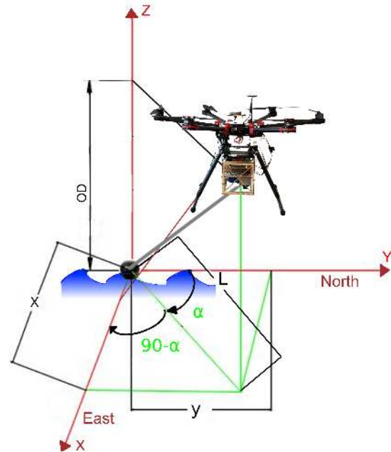
Figure 3. Sonar is the center of the reference system X, Y, Z . The horizontal displacement between the sonar and the drone is computed along the X and Y directions, while the vertical displacement is computed along the Z axis (object distance – OD). The angle \alpha is the azimuth, i.e., the angle between the Y axis pointing north and the vector between the drone and the sonar, projected onto the horizontal plane (in green). The azimuth angle is measured clockwise from north (i.e., \alpha is positive in the figure).
