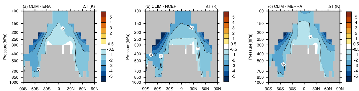
Figure 3. 5 yr (2006–2010) mean, zonally averaged differences between temperature simulated by the free-running CAM5 (“CLIM”) and the (a) ERA-Interim (ECMWF Interim Reanalysis), (b) NCEP (National Centers for Environmental Prediction Reanalysis), (c) MERRA (Modern Era-Retrospective Analysis for Research and Applications). Units: K. Regions with mean ice crystal number concentration lower than 5 \text{ g}^{-1} in the CLIM simulation are masked out in gray.
