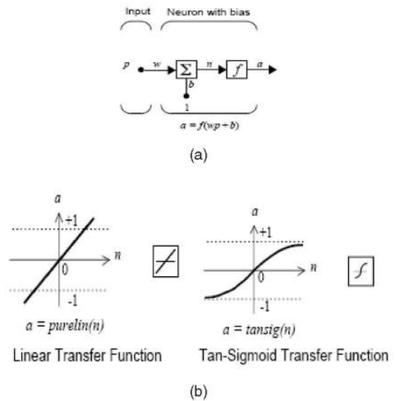
Fig. 3. Simple neuron and its transfer functions [25]. (a) Simple neuron with bias. (b) Two transfer functions.
