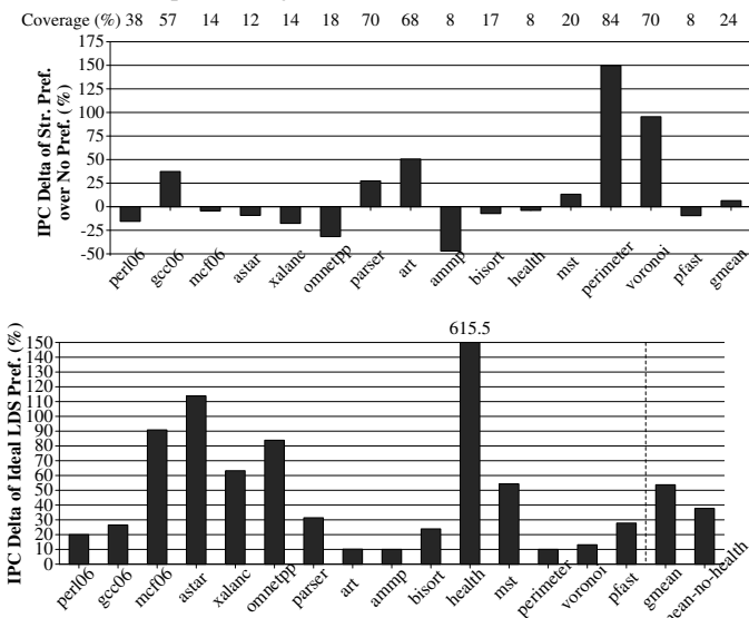
Figure 1. Potential performance improvement of ideal LDS prefetching
