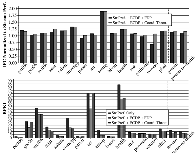
Figure 13. Prefetcher Throttling vs. Feedback Directed Prefetching
