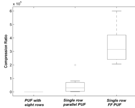
Fig. 16. The amount of CRP compressibility for parallel, FF and the proposed secure PUFs. Each box represents the results of 10 experiments on different PUF realizations.
