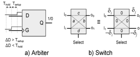
Fig. 1. PUF fundamental building blocks.
