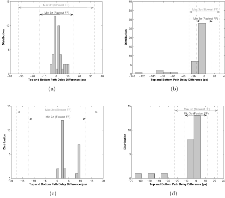
Fig. 25. The distribution of delay difference between the top and bottom paths. The distribution is calculated for 8 input challenges, 5 XC5VLX50 chips, and 3 XC5VLX110 chips. Figures (a) and (b) show the distribution for rising and falling transition delays on XC5VLX50 chips. Similarly, Figures (c) and (d) show the distribution for rising and falling transition delays on XC5VLX110 chips. The vertical lines show the 3\sigma detection edges of slow and fast arbiters (FF).
