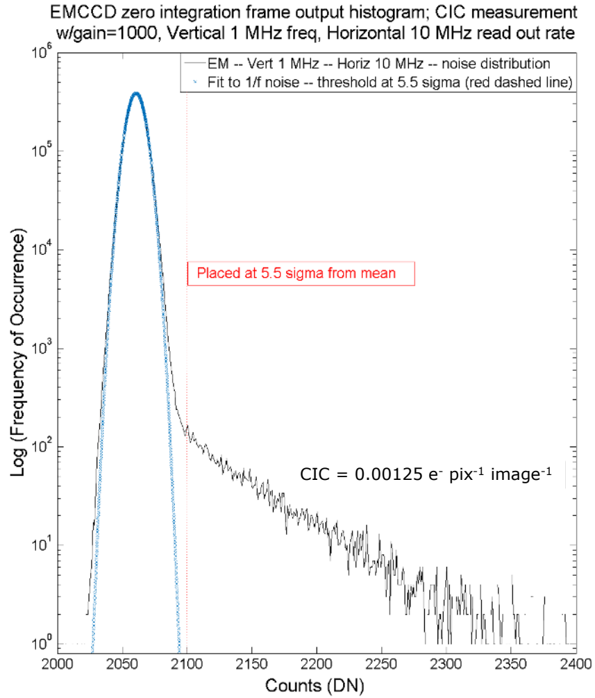
Figure 11. Histogram of 20 EMCCD frames, taken at a gain of 1000. The Gaussian function to the left is the read out noise (primarily 1/f ) with small amounts of CIC and dark current. The data points to the right of the 5.5\sigma are the total contribution of CIC, dark current and other spuriously generated charge. The 5.5\sigma threshold was applied to the mean of the blue Gaussian fit to the read out noise. When calculating CIC, we integrate under this curve, and scale by the total number of pixels per given image, and remove the dark current for this temperature. The result is charge generated from CIC and other spurious sources.
