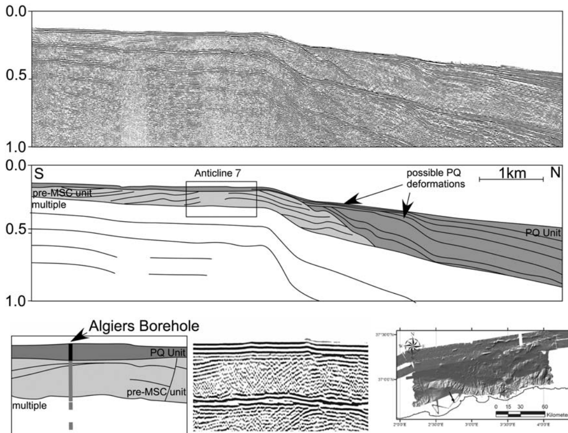
Figure 11. Line drawing of a 24-channel seismic reflection profile across the Khair al Din bank, west of Algiers (location in Figure 3). Age of the formation on seismic section is given by the projection of the Algiers borehole [Buroillet et al. , 1978] on the seismic section. Vertical exaggeration is 3× at the seafloor.
