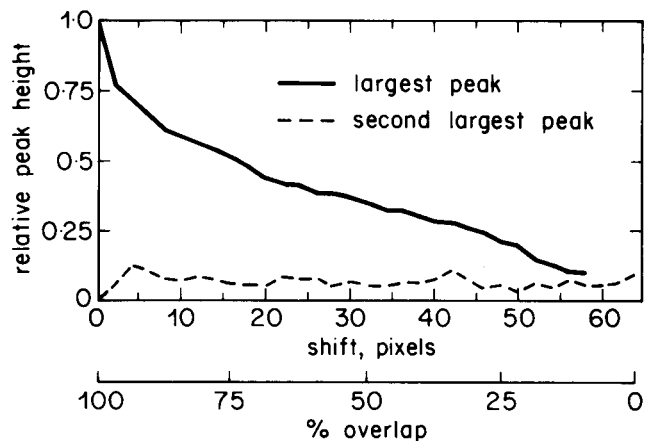
Fig. 4 - Correlation peak height as a function of shift size for a picture portion 64 pixels square from 'Pond' (integral pixel shifts only).
