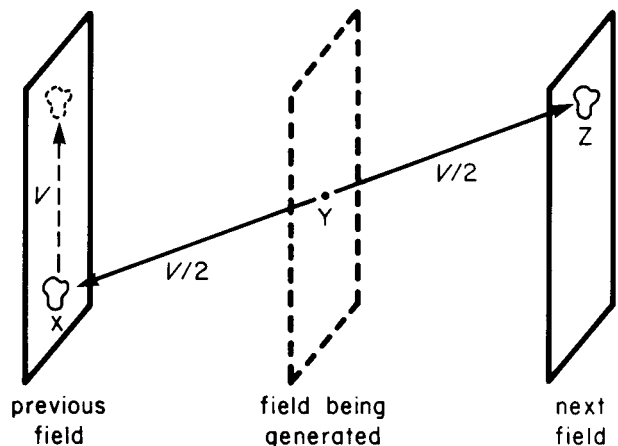
Fig. 16 - Generating an intermediate picture using simple motion compensated temporal interpolation.
