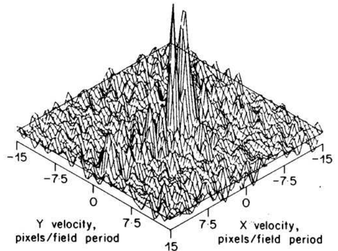
Fig. 15 - Correlation surface for a part of the 'Voiture' sequence for the small rectangular area indicated in Fig. 14.
