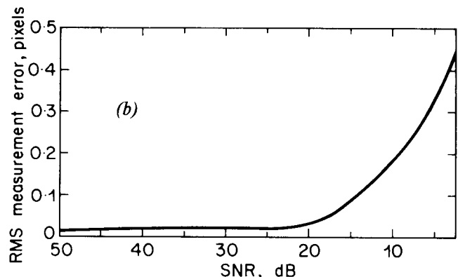
Fig. 11 - The effect of noise on (a) correlation peak height and (b) measurement error.
