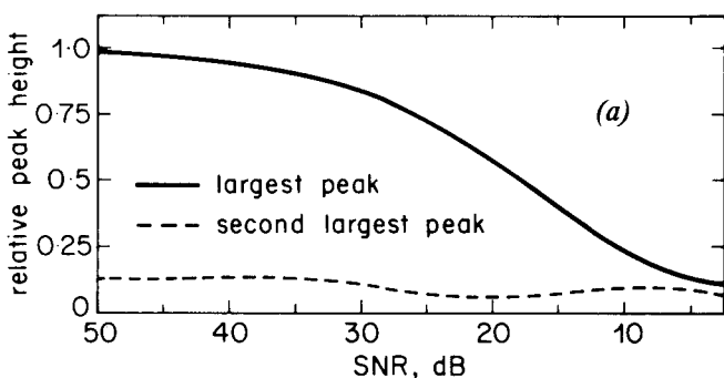
Fig. 11 - The effect of noise on (a) correlation peak height and (b) measurement error.
