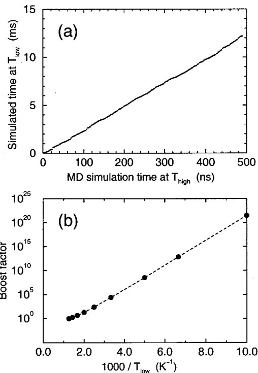
FIG. 3. Results from TAD simulations of an adatom hopping on a Ag(100) surface. Simulation parameters: T_{\text{high}}=800 K, \nu_{\text{min}}=2 \times 10^{12} \text{ s}^{-1} , and \delta=0.001 . (a) Simulated time at T_{\text{low}}=300 K as a function of the MD simulation time at T_{\text{high}} . A total of 398 adatom hops was recorded during a time of 12.2 ms at T_{\text{low}} . (b) Boost factor as a function of the reciprocal of T_{\text{low}} .
