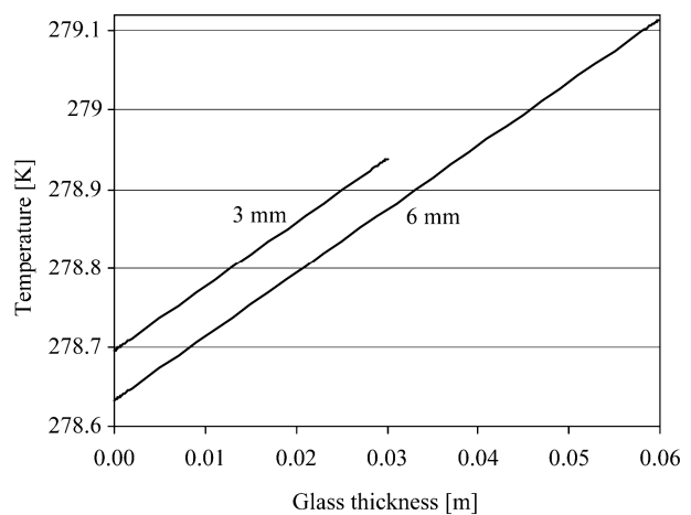
Figure 5. Temperature distribution within the single glazing window.
