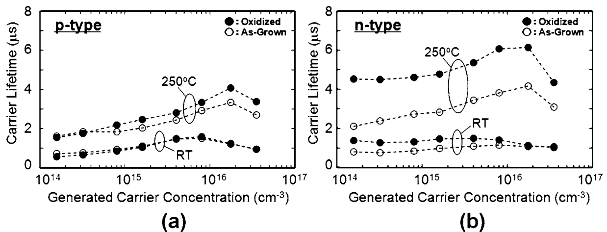
FIG. 5. Comparison of injection level dependencies of carrier lifetimes for 50 \mu\text{m} thick (a) p-type and (b) n-type 4H-SiC epilayers before (as-grown) and after thermal oxidation.
