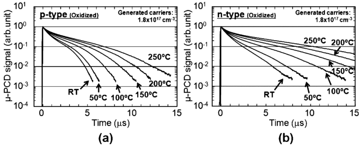
FIG. 4. PCD curves measured after thermal oxidation process for 50 \mu\text{m} thick (a) p-type and (b) n-type epilayers at the same location as Fig. 3 at various temperatures. The excitation intensity is 1.8 \times 10^{17} \text{ cm}^{-3} .
