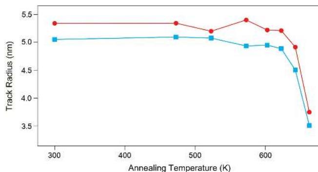
Figure 3 Ex situ annealing of tracks in apatite formed under 633 \text{ K} (high-T, circles) and 300 \text{ K} (RT, squares). At each temperature the samples were annealing for 20 min. The radius for both samples remains stable up to a temperature of 623 \text{ K} .
