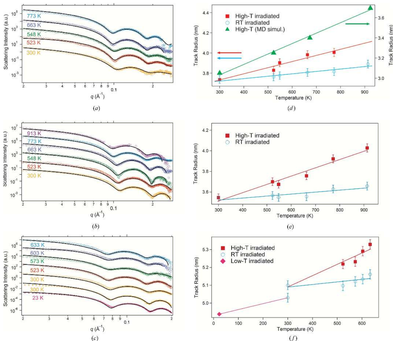
Figure 2 SAXS scattering intensities of ion tracks in quartz (a) \parallel c and (b) \perp c for different irradiation temperatures (open circles). (c) SAXS intensities for apatite \parallel c irradiated with 2.2 GeV (open circles) and 1.7 GeV (crosses) Au ions. A hard cylinder model was used to fit the results (solid lines). Spectra are offset for clarity. Typical intensity for each spectra at q = 0 is between 10 and 30 \text{cm}^{-1} . Track radius in quartz (d) \parallel c and (e) \perp c for high-T (filled squares) and the corresponding reference samples that underwent the same heat cycle (open circles). In (d) the right ordinate shows an MD simulation for ion tracks (filled triangles). Both vertical axes show the same scale. (f) Track radius in apatite \parallel c as a function of irradiation temperature for high-T (filled squares) and 23 K (filled diamonds) and as a function of annealing temperature for the reference samples (open circles).
