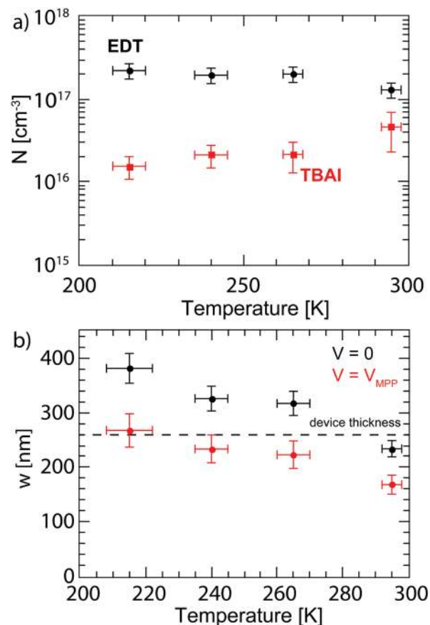
Fig. 7 (a) Doping concentration of EDT (black dots) and TBAI (red squares) capped PbS measured by Mott–Schottky analysis. The error bars are determined by the uncertainty in permittivity, slopes of the Mott–Schottky curves, and temperature. (b) Depletion width calculated at zero bias (black) and at the maximum power point (red). The dashed line shows the device thickness. The error bars originate from the uncertainty in the permittivity and doping concentrations.
