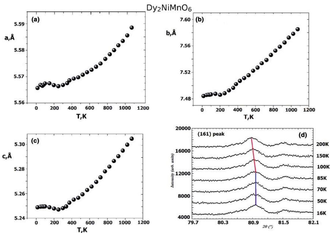
Fig. 2 a–c Temperature dependence of the lattice parameters for Dy 2 NiMnO 6 extracted from the XRPD patterns. The temperature evolution of the (161) reflection is shown in (d)
