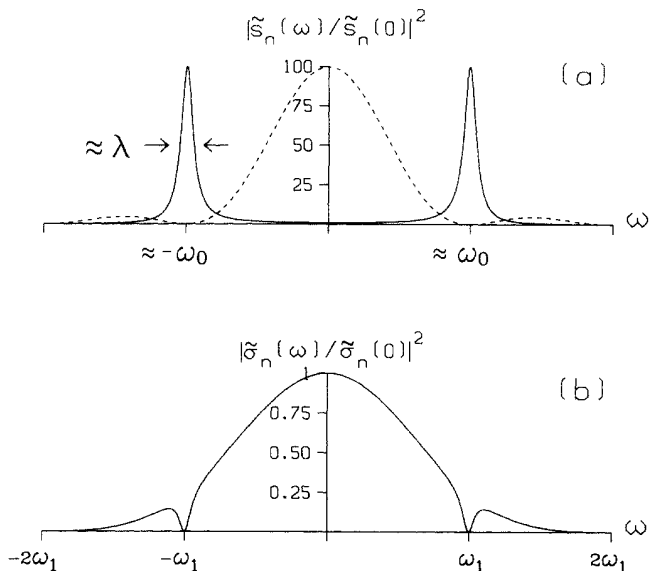
FIG. 1. (a) Power spectrum of the noise before averaging, |\bar{x}_n(\omega)|^2/|\bar{x}_n(0)|^2 (solid), and 100 [\sin(\pi\omega/\omega_1)/(\pi\omega/\omega_1)]^2 (dashed). (b) Power spectrum of the resulting noise, |\bar{\sigma}_n(\omega)|^2/\omega_0 = 10^{12} \text{ s}^{-1} , and \lambda = 10^{11} \text{ s}^{-1} .
