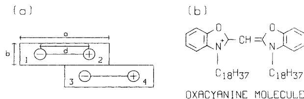
FIG. 2. Left: brickstone work representation of a monolayer Scheibe aggregate, with each molecule represented as an extended dipole. Right: oxycyanine molecule.
