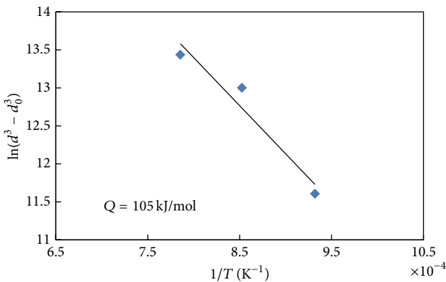
FIGURE 9: Arrhenius plot of \text{CeO}_2 nano-grain size versus 1/T showing the exhibited activation energy in the temperature range of 1073 K to 1273.
