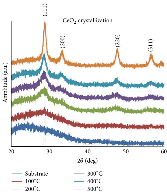
FIGURE 2: XRD intensity peaks from precipitated powders showing the effect of temperature on the transition from amorphous to crystalline nano- \text{CeO}_2 .
