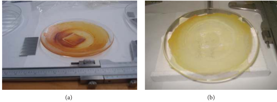
FIGURE 1: (a) \text{Ce}(\text{OH})_4(\text{s}) precipitated just after the drying stage and (b) nanocrystalline \text{CeO}_2 after annealing at 573 K for 60 minutes.
