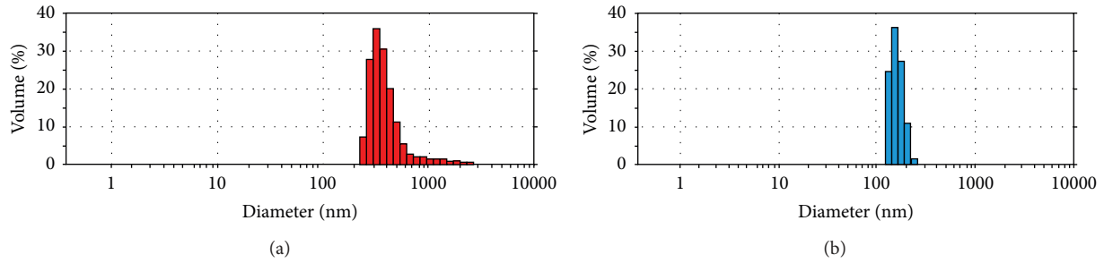
FIGURE 4: (a) Size distribution of nano-CeO 2 agglomerates after precipitation synthesis and (b) after 10 minutes of ultrasonic dispersion.
