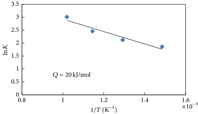
FIGURE 8: Arrhenius plot of \text{CeO}_2 nanograin size versus 1/T showing the exhibited activation energy at low temperatures (673 K to 973 K) using data from Ivanov et al. [13].
