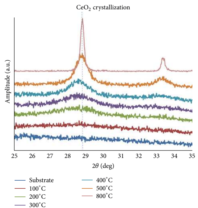
FIGURE 3: XRD intensity peaks associated with the recrystallization of \text{CeO}_2 powders and the effect of temperature on peak shifting and broadening.
