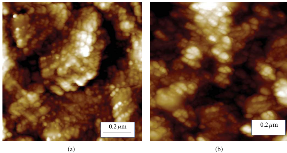
FIGURE 5: AFM micrographs showing (a) morphology of the as-synthesized nano-CeO 2 particle agglomerates and (b) effect of the ultrasonic dispersion on breaking the particle clusters.
