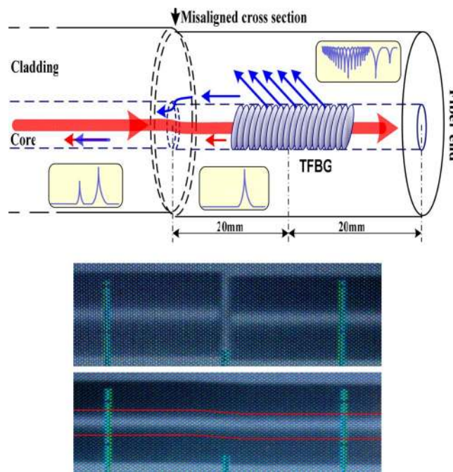
Fig. 1. (Color online) Schematic diagram of a TFBG with a misaligned fusion for vibration measurement and before and after photographs of the fusion splice.
