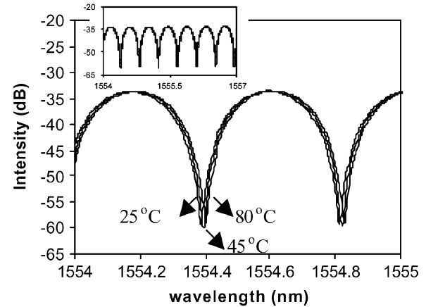
Fig. 2. Transmission spectra as a function of temperature for the HiBi-PCF-FLM. Inset: Transmission spectra in the range of 1554–1557 nm.
