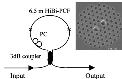
Fig. 1. Experimental setup of HiBi-FLM. Inset: Micrograph of the HiBi-PCF.
