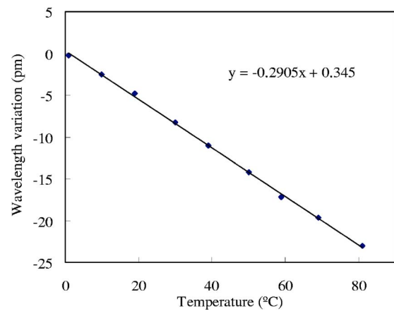
FIG. 5. (Color online) Wavelength variation of the transmission minimum at 1547 nm against temperature.
