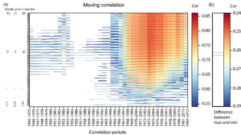
Figure 7. (a) Thirty-year moving correlation from 1945 to 2012 between the monthly mean of daily maximum temperature, from January of the current year (1, 0, 1) to December of the previous year (12, −1, 36) with a cumulative monthly mean from 1 to 36 months and the BasPois chronology. Red numbers indicate the chosen climatological parameter: 9, September, −1, previous year, 21, months used for the cumulative monthly mean. (b) The four best parameters are represented. The reddish line indicates the least difference between the maximum and minimum correlation in the correlation periods.
