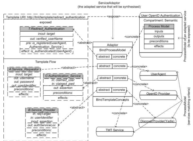
Fig. 12. Adapted service (exposed) is created via a transformation.
