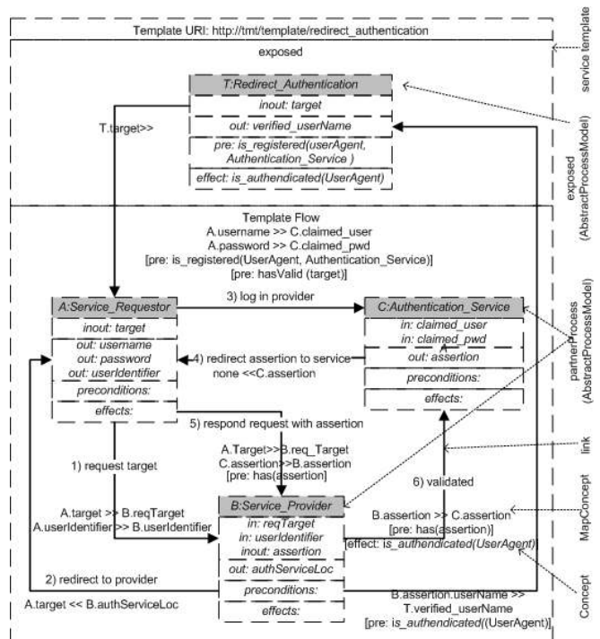
Fig. 8. Specifying a service template for redirecting authentication.
