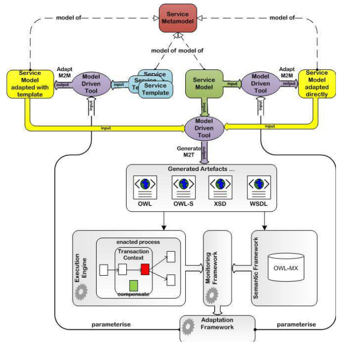
Fig. 6. Components realising the development process of our approach.
