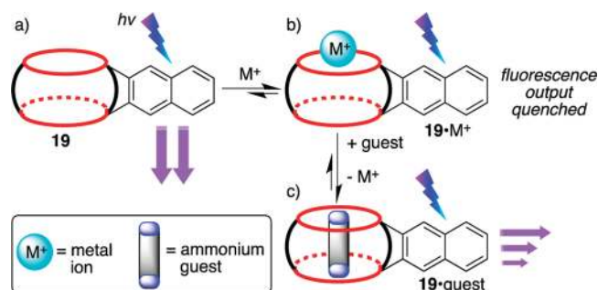
Scheme 4. Concept of Fluorescence Assay Based on Fluorescent CB[6]-Derivative 19 a
