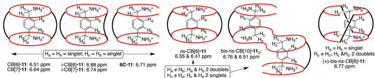
Figure 1. Illustration of the use of 11 as a probe of CB[ n ] reaction mixtures by ^1\text{H} NMR spectroscopy.
