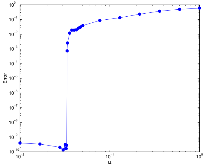
Fig. 2: Demonstration of the exact penalty property for the Dantzig selector. For \mu \leq \mu_0 \approx 0.025 , the solution to the smoothed model coincides with the original model to solver precision.
