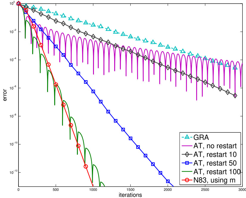
Fig. 5: First-order methods applied to a strongly convex problem: GRA, AT without restart, AT with restart, and N83 tuned with knowledge of the strong convexity parameter. The y -axis is \|x_k - x^*\|_2 / \|x^*\|_2 .
