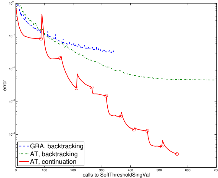
Fig. 10: Noisy matrix completion on a non-low-rank matrix, using various first-order methods. The \circ labels on the continuation line series indicate the iterations at which continuation occurred. The error is \|X_k - X^*\|_F / \|X^*\|_F .
