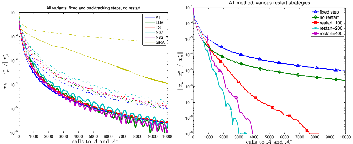
Fig. 6: Comparing first order methods applied to a smoothed Dantzig selector model. Left: comparing all variants using a fixed step size (dashed lines) and backtracking line search (solid lines). Right: comparing various restart strategies using the AT method.
