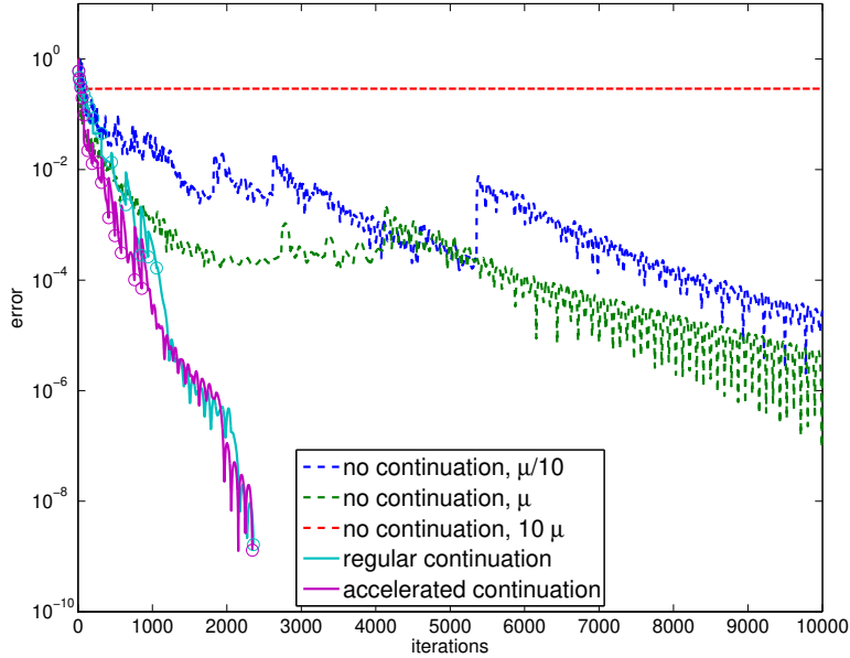
Fig. 4: Comparing fixed smoothing and continuation strategies for a Dantzig selector model. The horizontal axis gives the number of inner iterations of each first-order method. For the two continuation strategies, the circles depict the completion of each continuation step.
