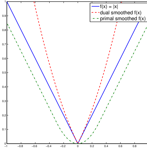
Fig. 1: The original objective f(x) = |x| (blue), our modification (red), and the Moreau-Yosida regularization [37] (green) used in [5, 53].
