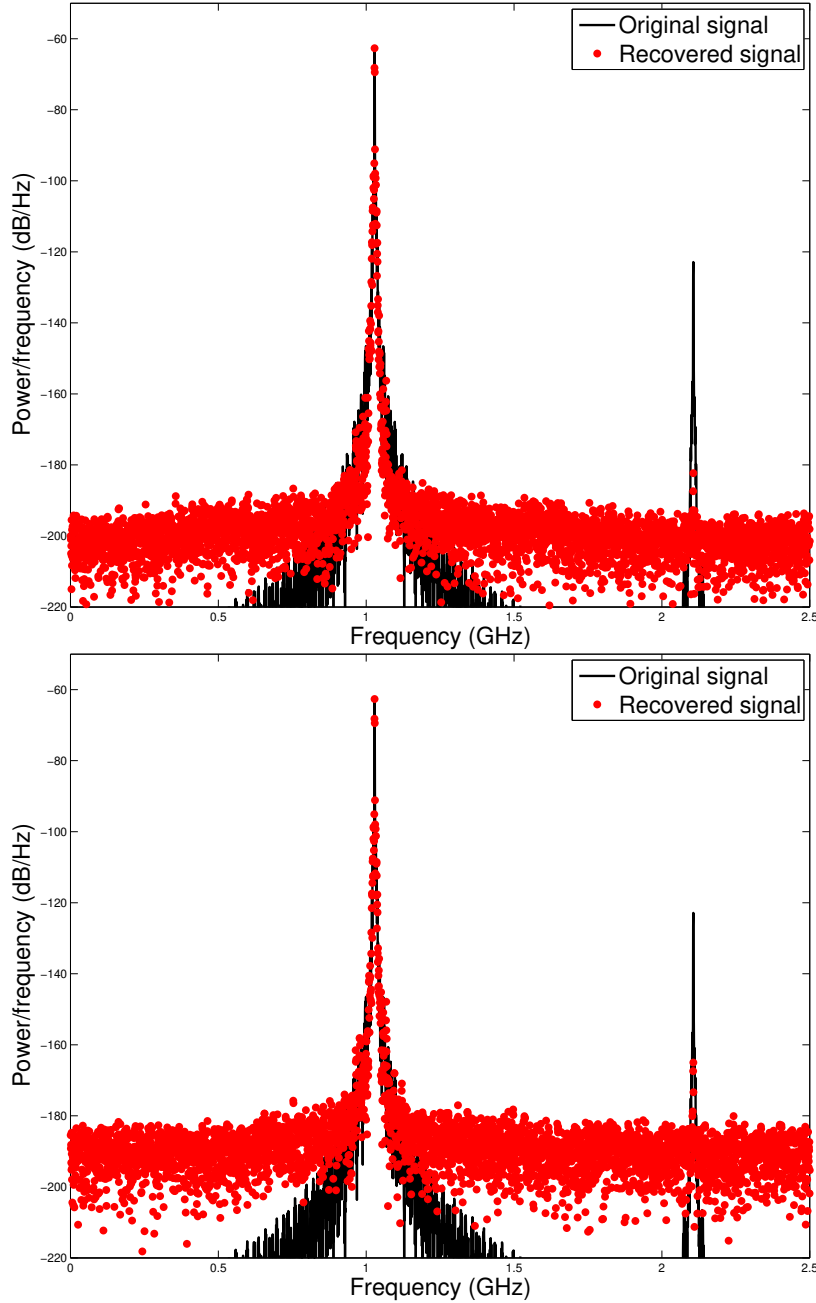
Fig. 11: Recovery of a small pulse 60 dB below a large pulse. The first plot employs a Dantzig selector, the bottom employs LASSO.
