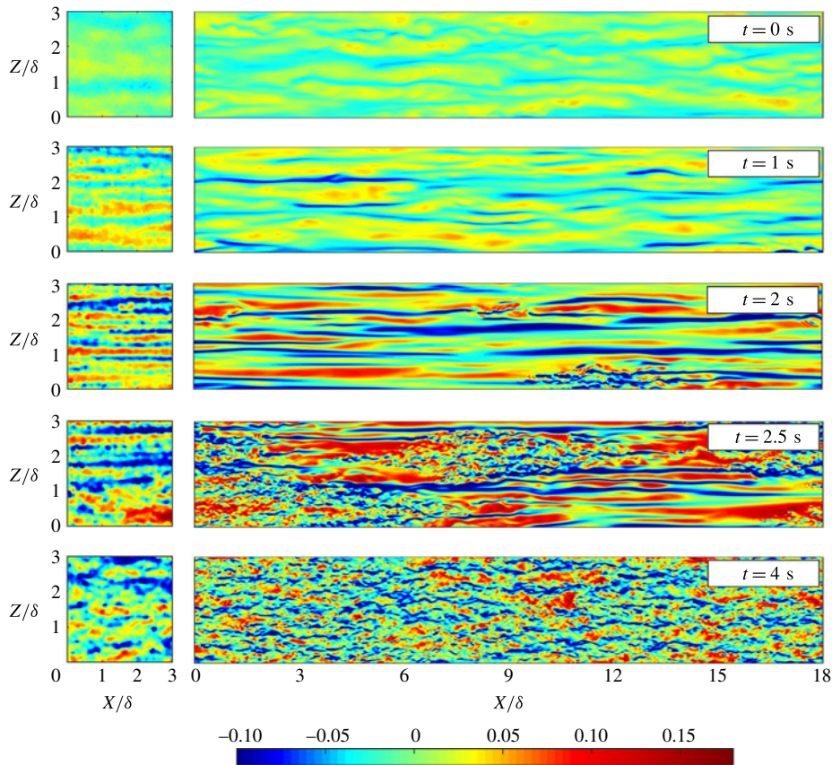
FIGURE 3. Distribution of the streamwise fluctuating velocity u' ( \text{m s}^{-1} ) over a horizontal plane close to the wall ( y = 2 \text{ mm} , y^{+0} = 15 , where y^{+0} = yu_{\tau 0}/\nu with y being the distance from the wall and u_{\tau 0} the friction velocity of the initial flow) at several instants of the transient flow of case A2. The PIV measurements are on the left and the LES results are on the right.
