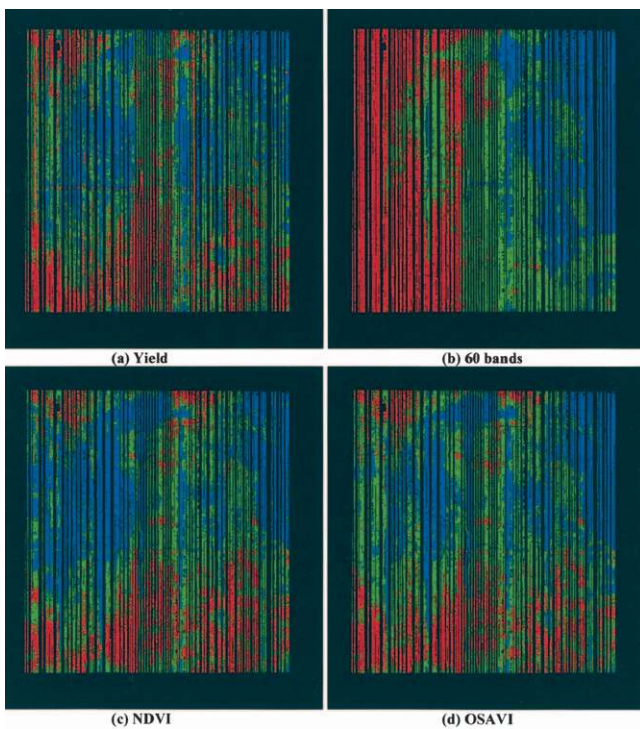
Fig. 7. Unsupervised K means clustering method for low (red)-, medium (green)-, and high (blue)-yield classes calculated from the hyperspectral airborne image that obtained the highest correlation with yield (5 July 2001). It shows better performance for OSAVI than NDVI index, with poor segmentation performance when 60 absolute reflectance bands are used. Airborne image pixels shown are only those where yield data were collected with the yield monitor.
