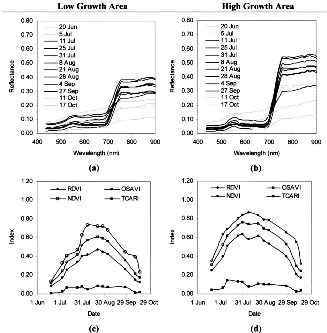
Fig. 4. Time series of (a and b) hyperspectral reflectance and (c and d) chlorophyll-related indices (TCARI), leaf area index related indices (RDVI and NDVI), and OSAVI calculated for areas of (a and c) low and (b and d) high growth development for the entire growing season.
