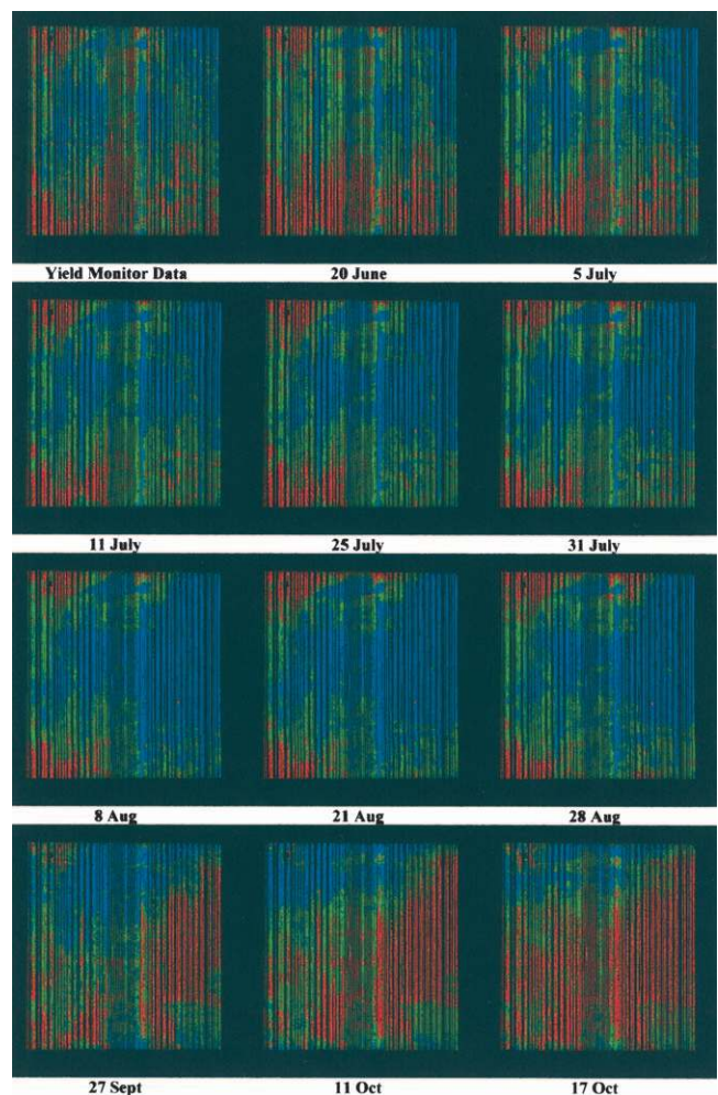
Fig. 8. Time series of segmented imagery using the OSAVI index for low (red)-, medium (green)-, and high (blue)-yield through K -means method, enabling the visual comparison with classes calculated from the spatial yield data. Airborne image pixels shown are only those where yield data were collected with the yield monitor.
