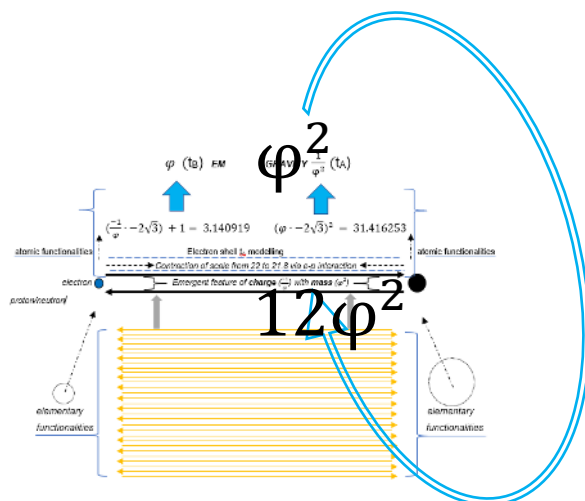
Paper 5, figure 4: \phi^2 \gg \gg 12 \phi^2, \phi^2 \gg \gg (\phi \cdot -2\sqrt{3})^2 , a process of the CMBR.
