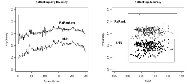
(a) Temporal Diversity (b) RMSE vs. Diversity
