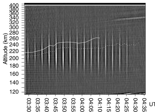
Figure 2. Altitude-time plot of background-subtracted 557.7 nm optical data from Poker Flat with the pump wave reflection (solid line) and upper-hybrid resonance (dotted line) altitudes overlaid. A spatial median filter has been applied, corresponding to \sim 4 min in the time domain and \sim 10 (25) km at low (high) altitudes.
