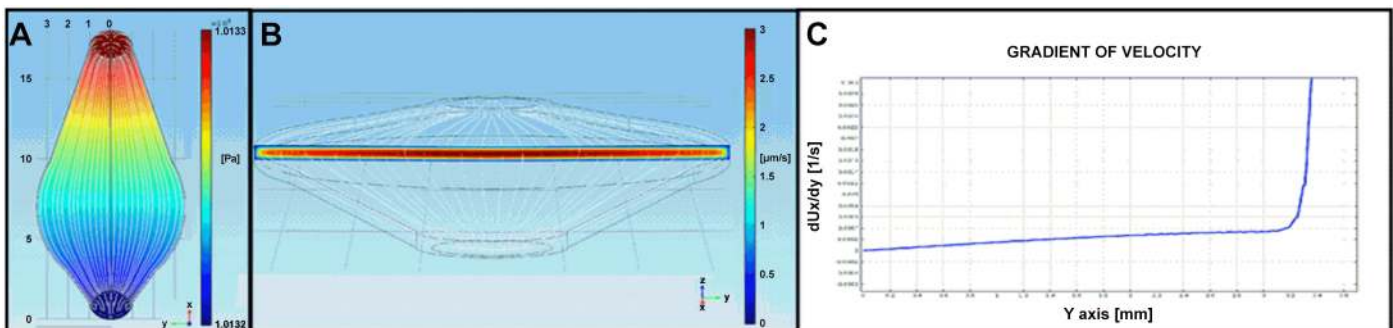
Fig 2. Simulation of the microfluidic flow in the chamber. a: Top view of the results of the simulation of half channel. Stream lines are represented in grey. The colours and the scale bar are relative to the pressure along the channel [Pa]. b: 3D view of the simulated system. Stream lines are represented in grey. A heat map of the values of the x component of the velocity in the widest section of the channel is reported together with the colour scale bar [ \mu\text{m/s} ]. c: Plot of the gradient of the x component of the velocity along the y-axis versus the distance from the centre of the channel.
